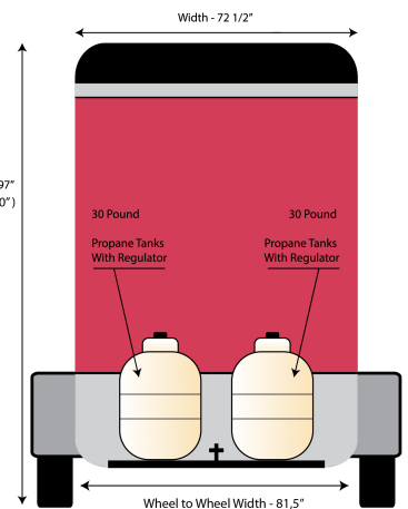
Outside Dimensions Back Side
