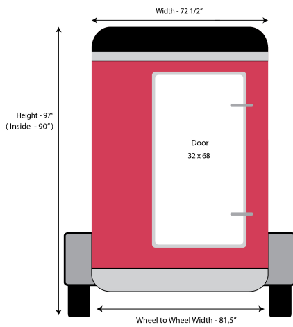
Outside Dimensions Front Side
